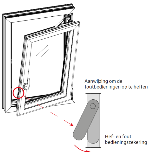
Figuur B1.1 Anti-foutbediening
